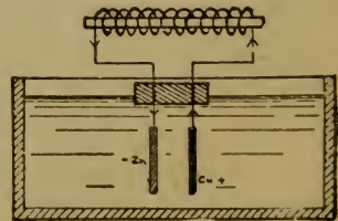
Figure 18 Floating helix and electromagnet.
